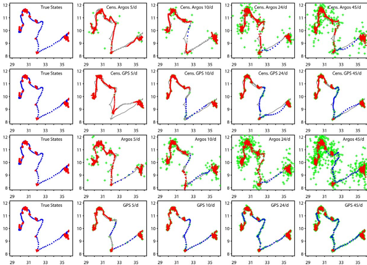
Fig. 2. Maps of SSM model fits to small scale (sea lion-like) simulated movement with rapid behavioral state switches to varying data qualities. X- and y-axis scales are arbitrary units but approximately equal to degrees of latitude and longitude. Green “+” are simulated observations, grey line the simulated track (shown with known state in the left column of panels). Location estimates are shown with color indicating inferred behavioral state. Blue is “transit”, red “resident”, and grey unclassified.
