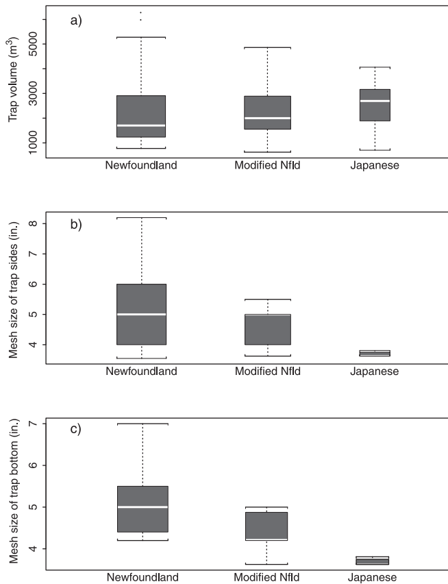
Fig. 5. Box-and-whisker plots showing differences in the (a) volume and (b) side and (c) bottom mesh sizes of Newfoundland, modified Newfoundland, and Japanese cod traps in the northern cod inshore fishery. See text for details of cod trap designs. Medians are represented by white bars in each box, the lower and upper ends of each box represent the 25 and 75% quartiles, respectively, the whiskers represent lines extending from the top and bottom of each box to adjacent data no more than 1.5 times the interquartile range, with values beyond this range indicated by solid circles, and the width of each box is proportional to the square root of the number of traps represented in each sample.
