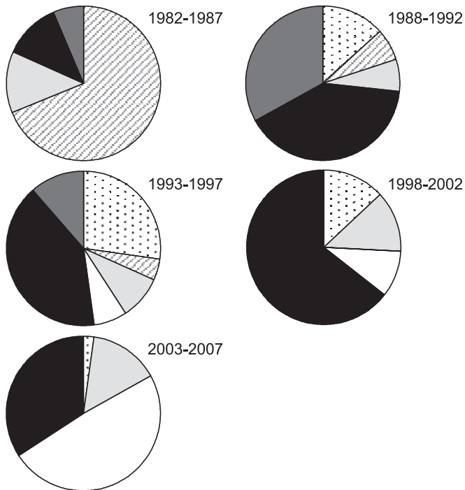
Fig. 3. Proportional representation of research contributions by Ram Myers for each of six research themes: life history evolution (hatched area), oceanography (dark grey), recruitment variability (stippled area), conservation biology (open), population modelling (solid), and general biology (light grey).
