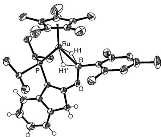
Fig. 4 ORTEP diagram for 8 (featuring one of the two disordered components of the isopropyl fragments) shown with 50% displacement ellipsoids and with selected H atoms omitted for clarity.
