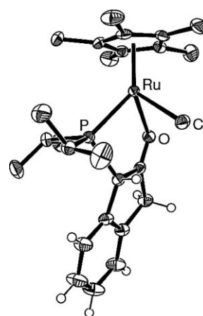
Fig. 1 ORTEP diagram for 2·0.5C 6 H 6 shown with 50% displacement ellipsoids and with selected H atoms and the benzene solvate omitted for clarity.
