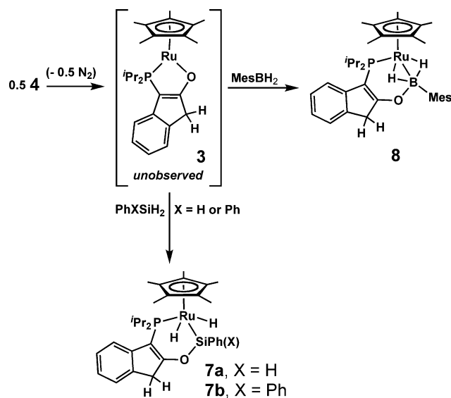
Scheme 3 Reactions of putative 3 with PhXSiH 2 and MesBH 2 (X = H or Ph; Mes = 2,4,6-trimethylphenyl).
