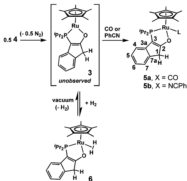
Scheme 2 Reactions of putative 3 leading to the 3 ·L adducts 5a,b and 6 (the indenyl numbering convention is provided for 5 ).
