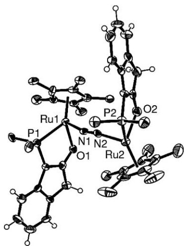
Fig. 2 ORTEP diagram for 4 shown with 50% displacement ellipsoids and with selected H atoms and the isopropyl methyl groups omitted for clarity.
