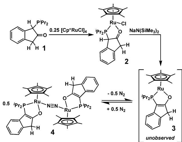
Scheme 1 Synthesis of 2 and the proposed interconversion of 3 and 4 .
