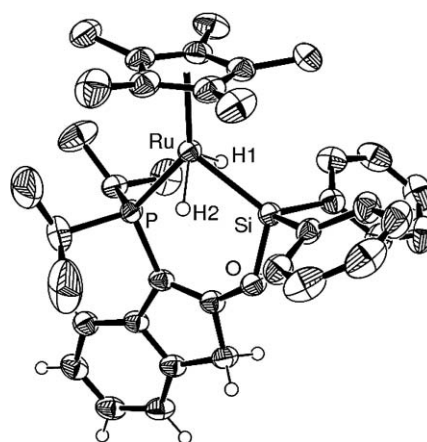
Fig. 3 ORTEP diagram for 7b shown with 50% displacement ellipsoids and with selected H atoms omitted for clarity.
